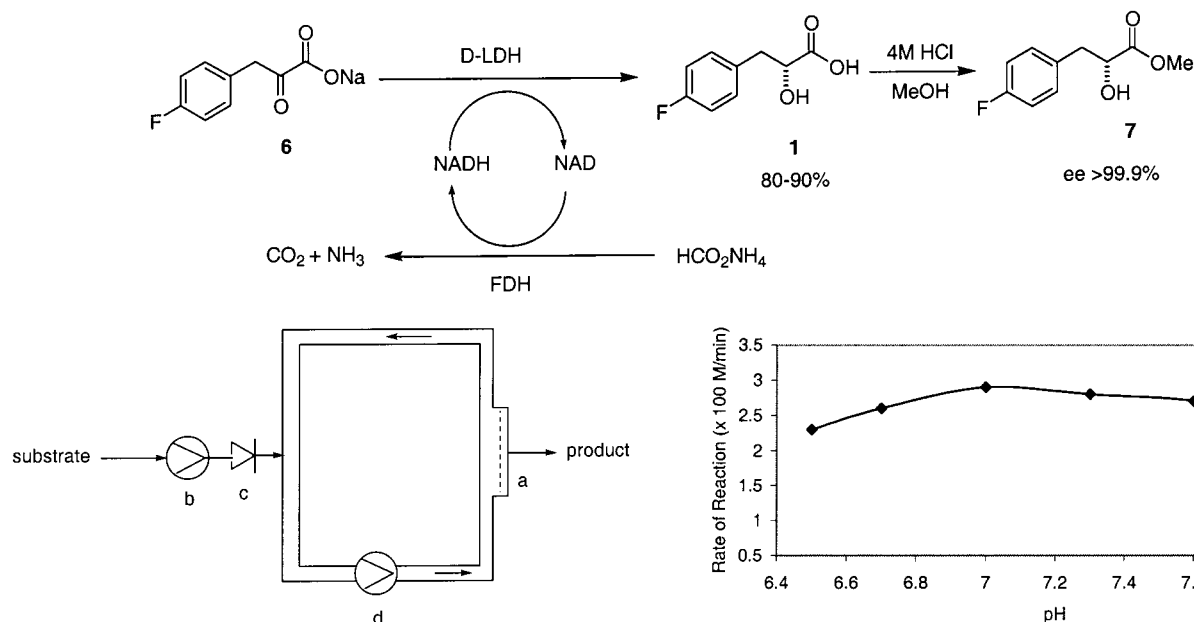
Figure 1. Schematic drawing of the enzyme membrane reactor.
